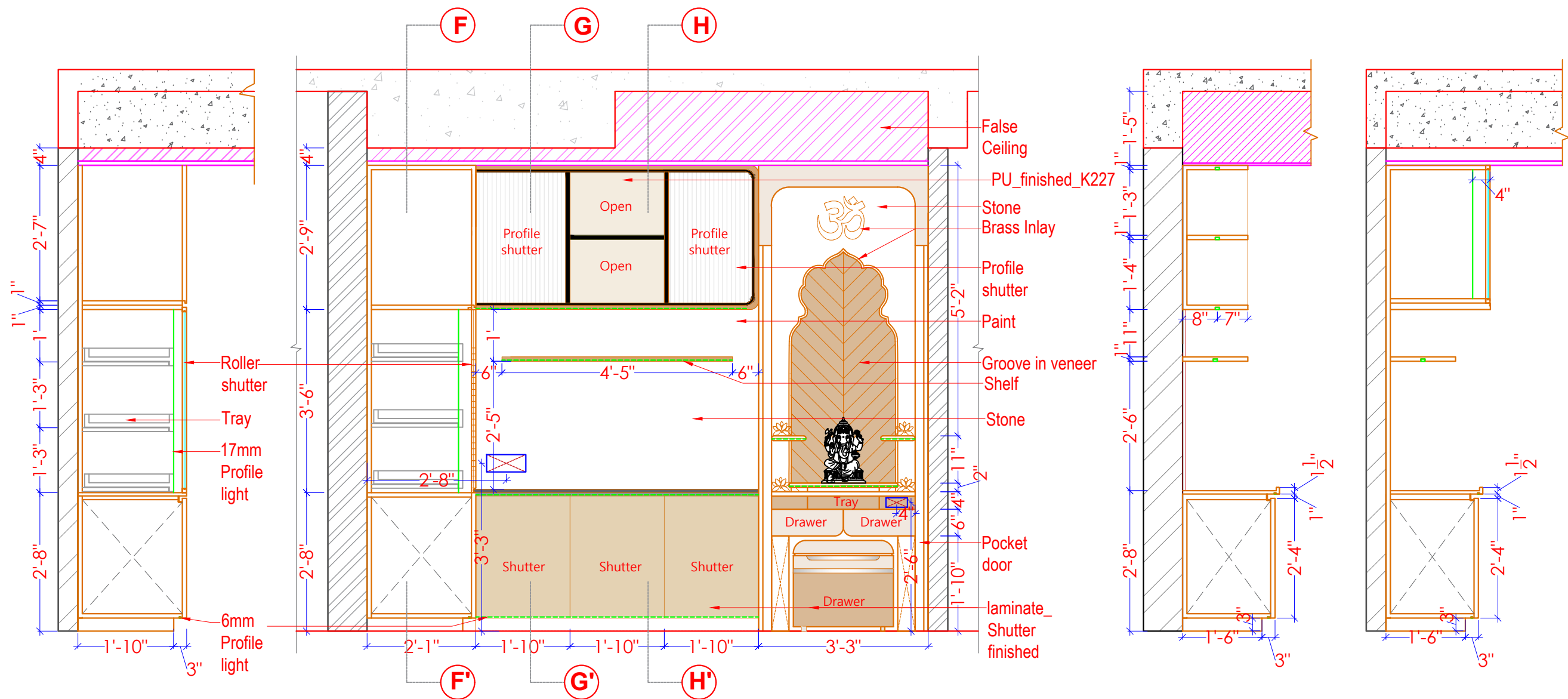
SECTION FF'
