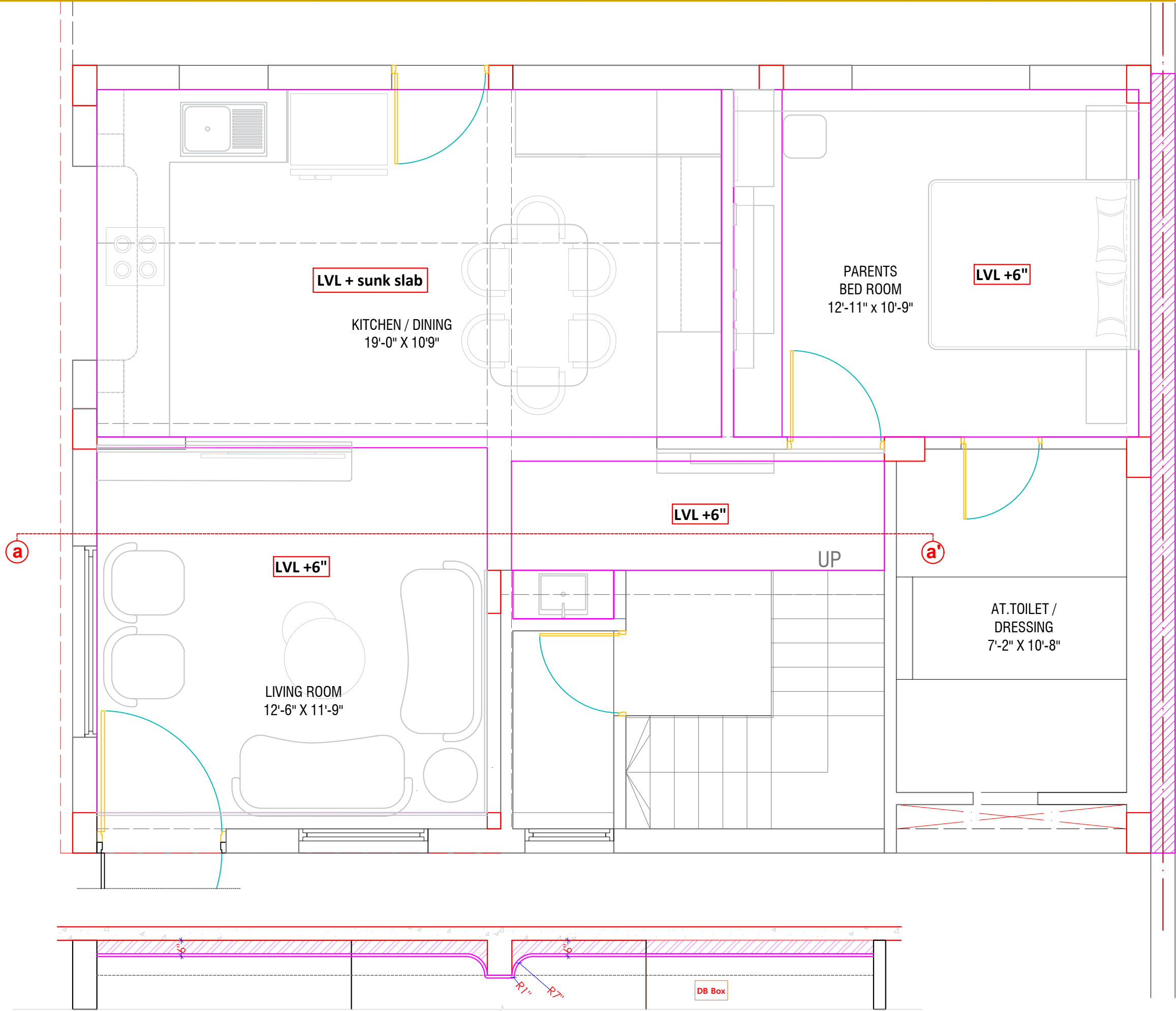
SECTION aa' FALSE CEILING LAYOUT
