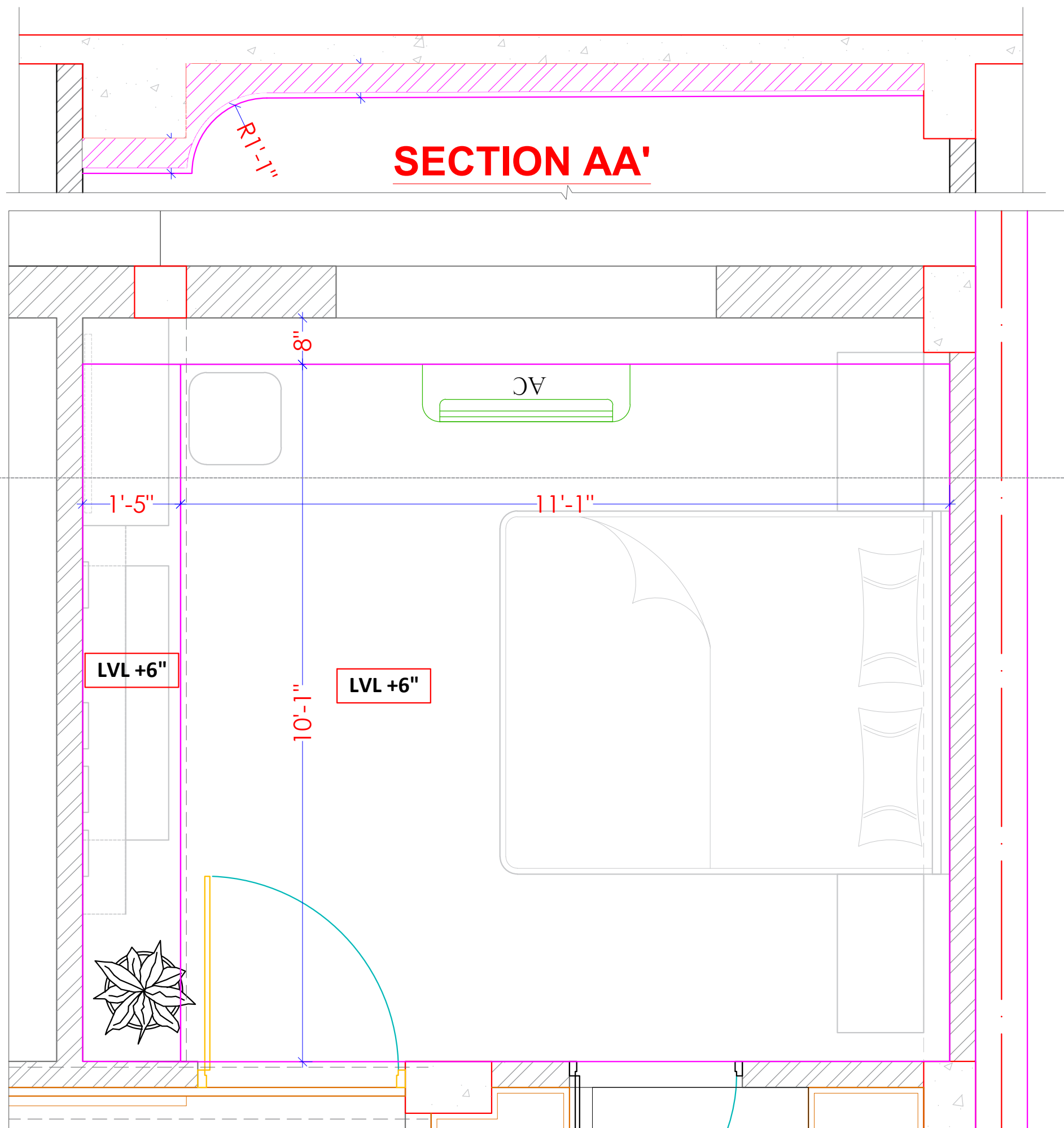
FALSE CEILING LAYOUT
