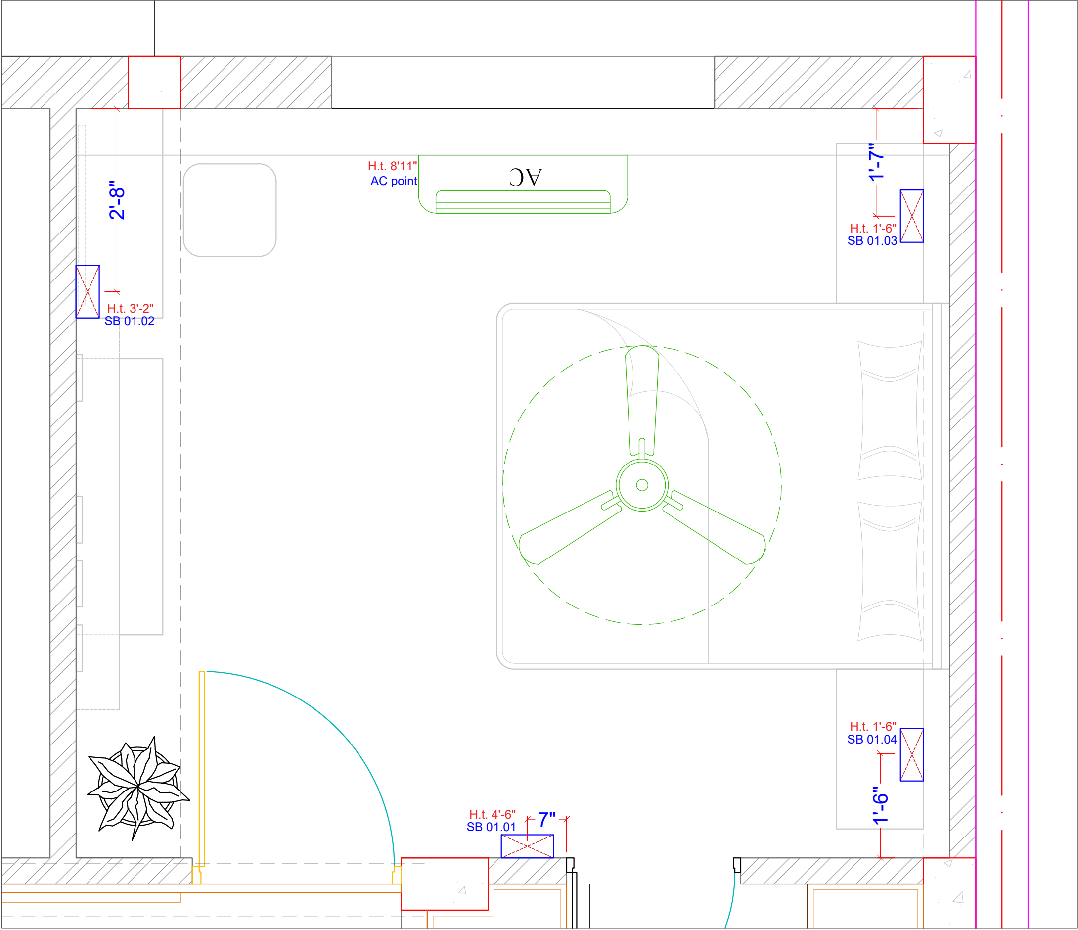
SWITCH BOARD LAYOUT
