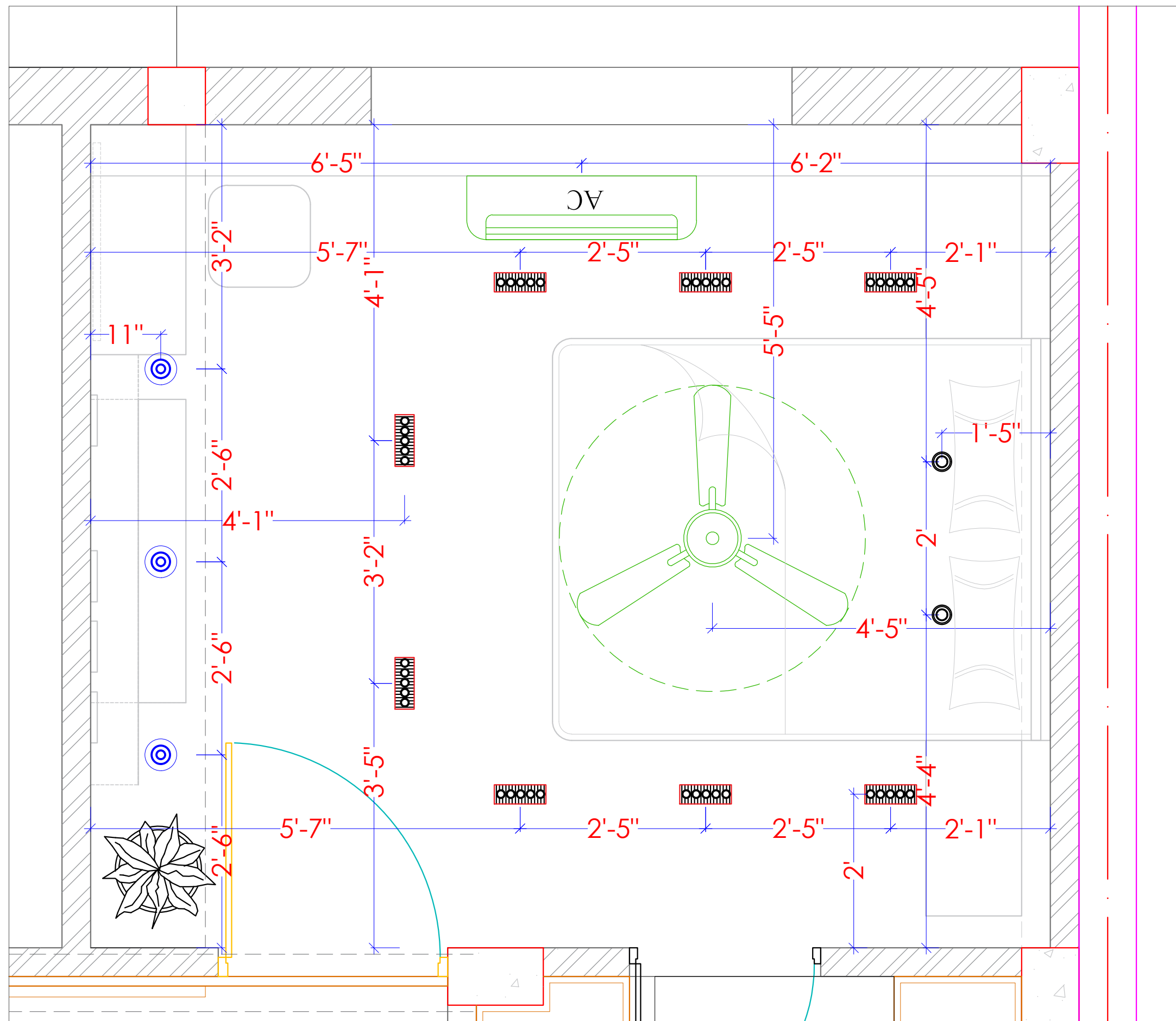
LIGHTING LAYOUT
