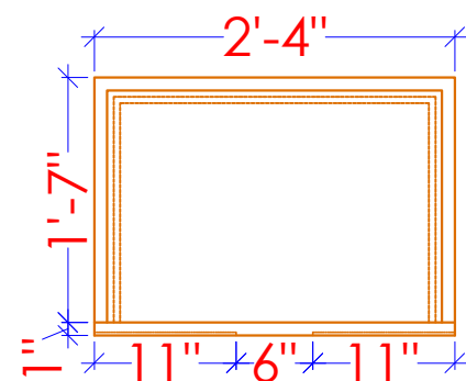
SIDE TABLE PLAN
