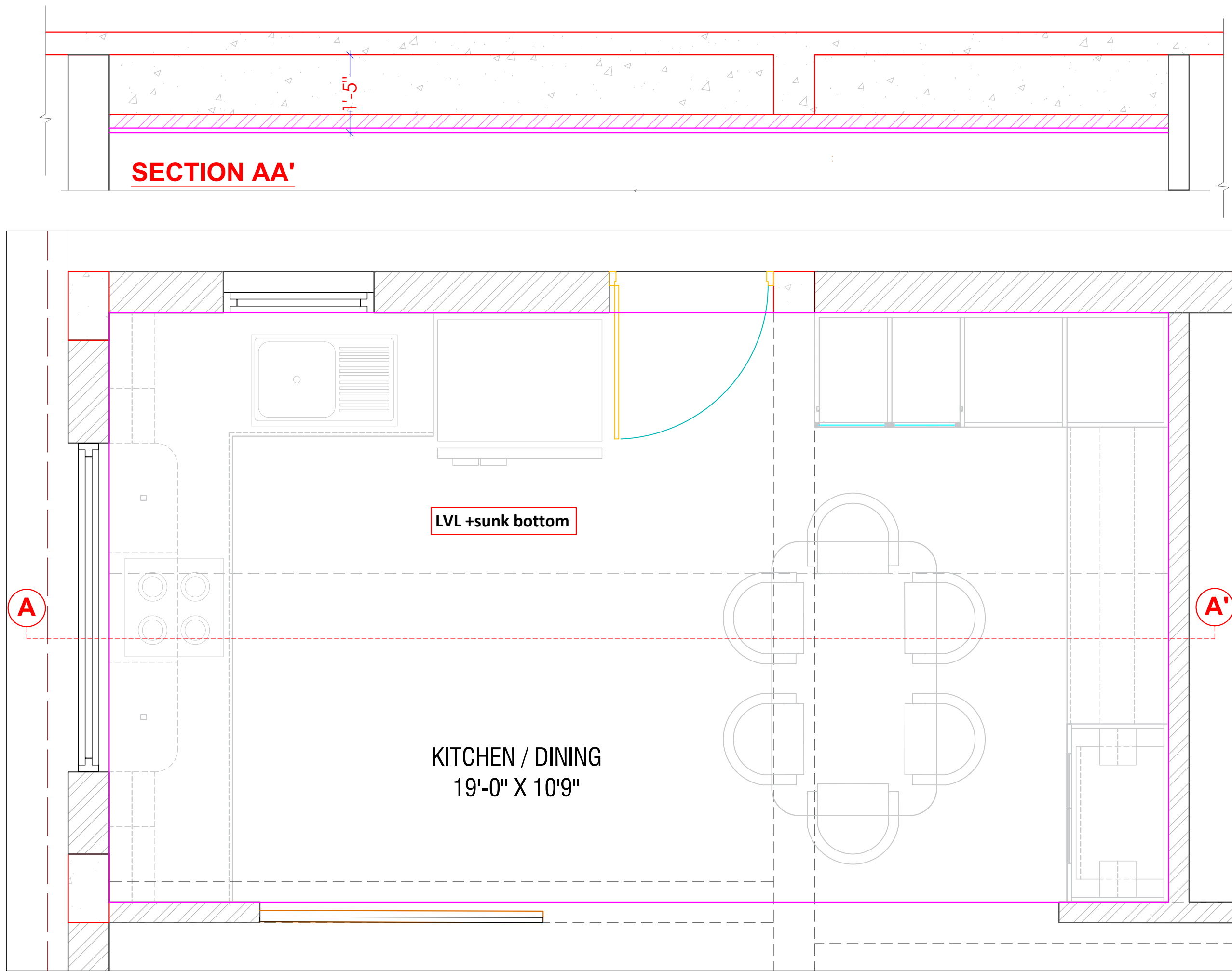
FALSE CEILING LAYOUT
