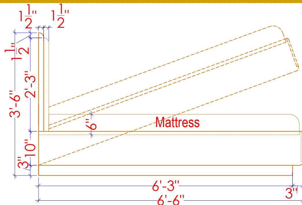
BED SIDE ELEVATION
